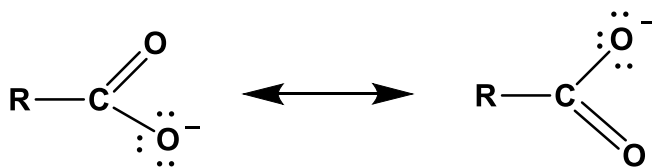
Resonance structures of Carboxylate Ion
