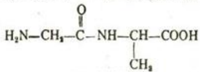
glycyalalanine
