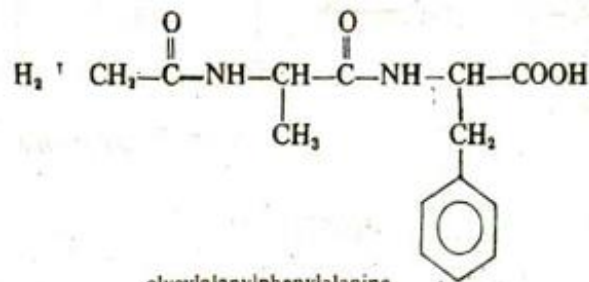
glycyalanylphenylalanine
